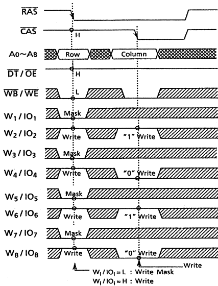
Figure 2. Write-per-bit timing cycle
