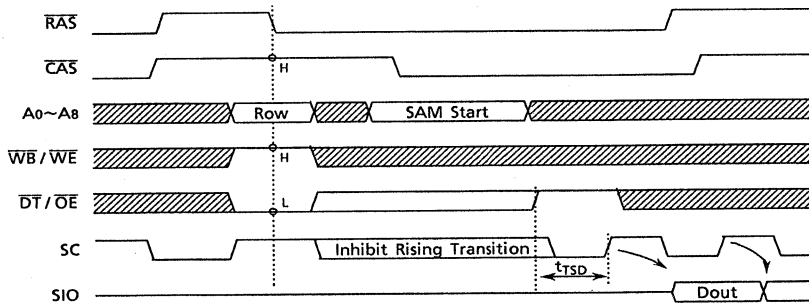
Figure 6. Read Transfer Timing
