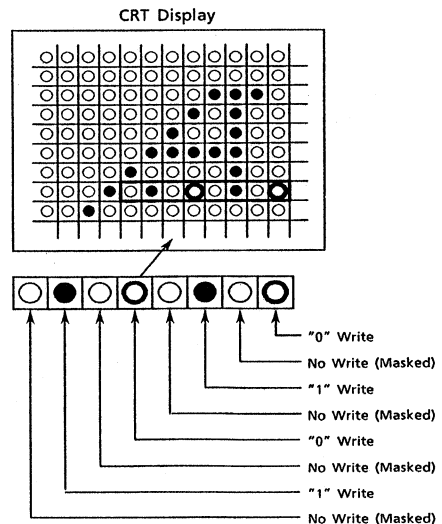
Figure 3. Corresponding bit-map
