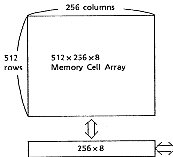
Figure 4. Data Transfer
