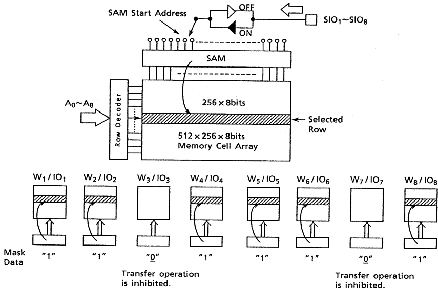
Figure 9. Block Diagram for Write Transfer Operation
