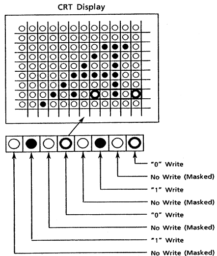
Figure 3. Corresponding bit-map
