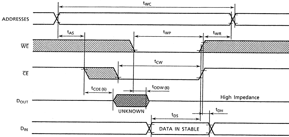
WRITE CYCLE2 (5) ( \overline{CE} Controlled Write)
