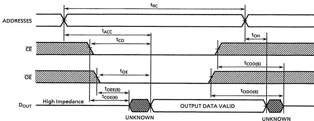
READ CYCLE (2)
