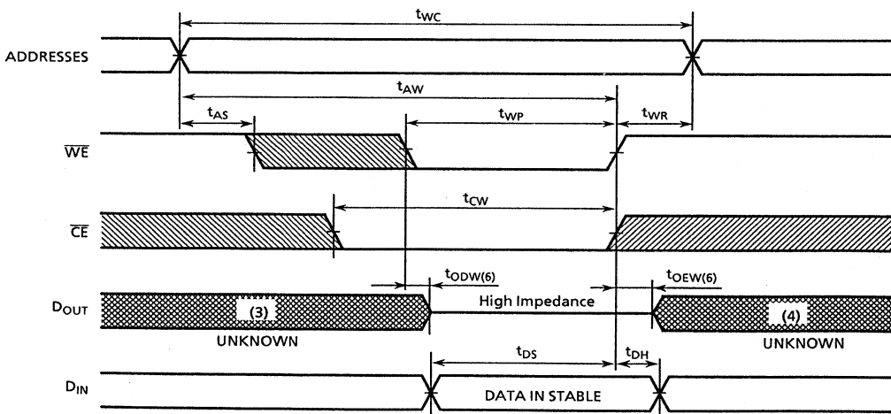
WRITE CYCLE1 (5) ( \overline{WE} Controlled Write)
