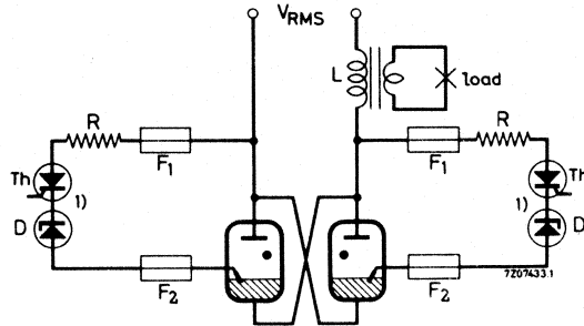
Anode excitation with individual thyristors
