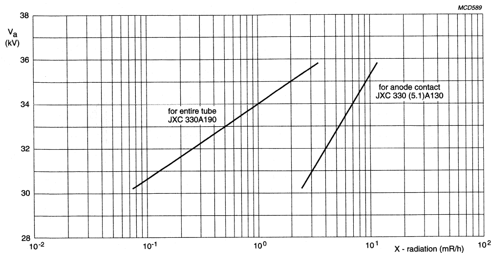
Fig.23 X-radiation limit curves at a constant anode current of 300 \mu A.
