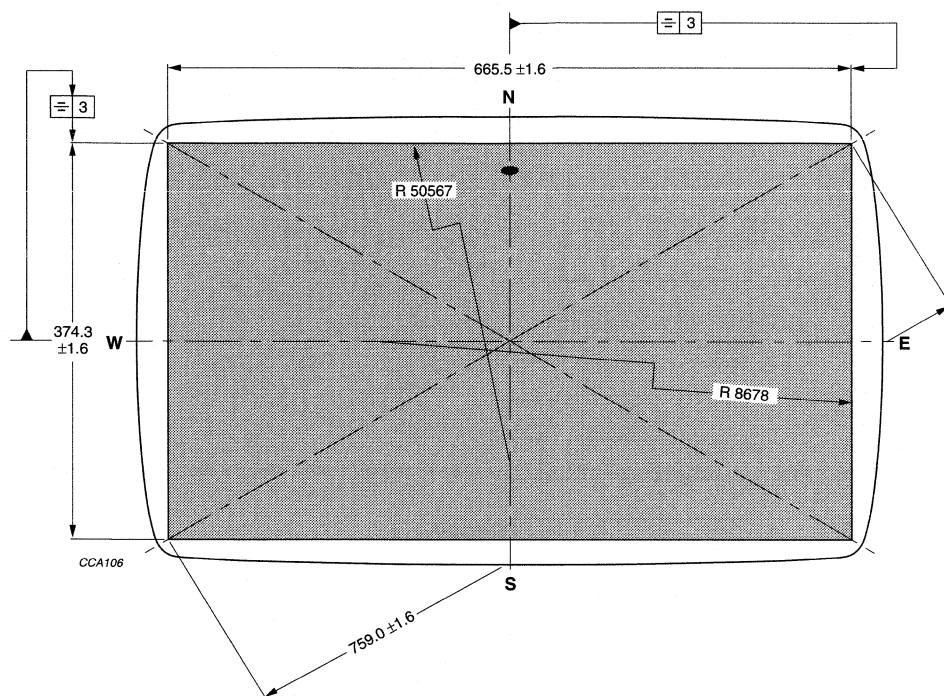
Fig.3 Phosphor dimensions.
