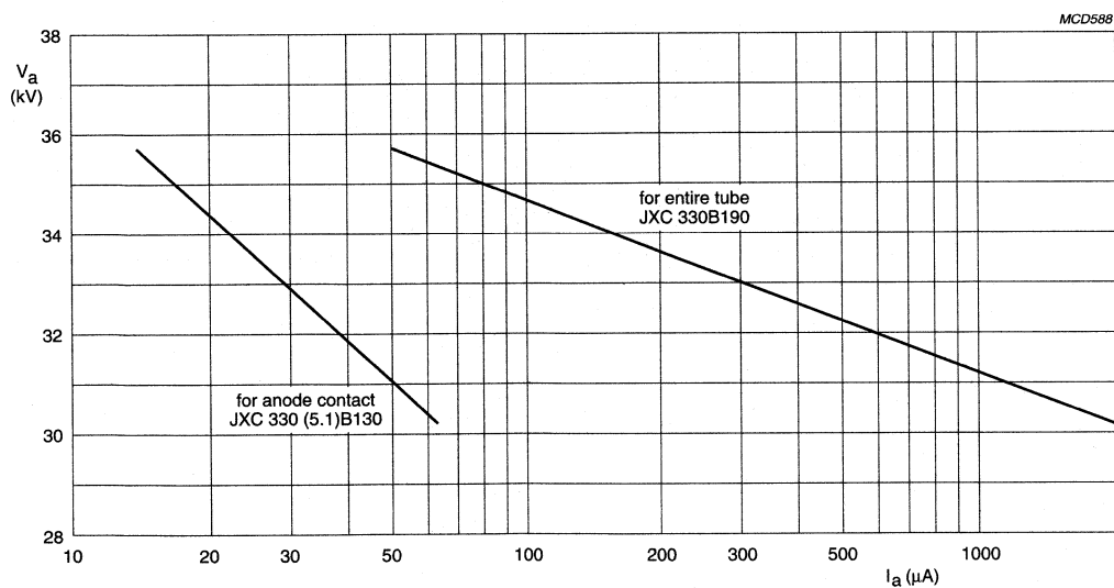
Fig.24 0.5 mR/h iso-exposure-rate limit curves.
