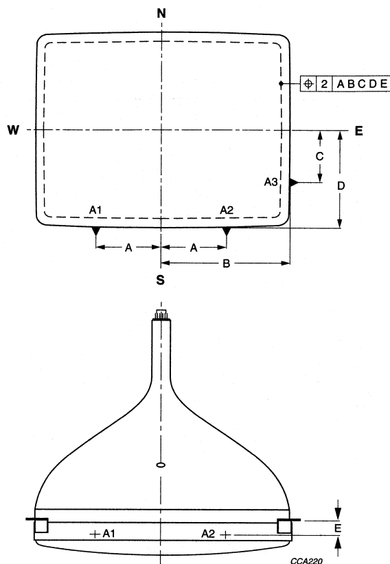
Fig.14 Phosphor alignment.
