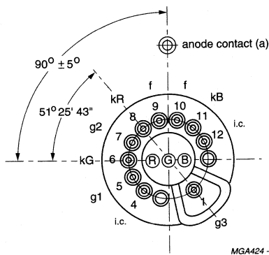
Fig.10 Pin configuration.
