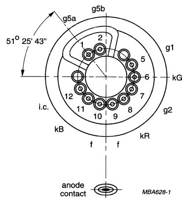
Fig.7 Pin arrangement.
