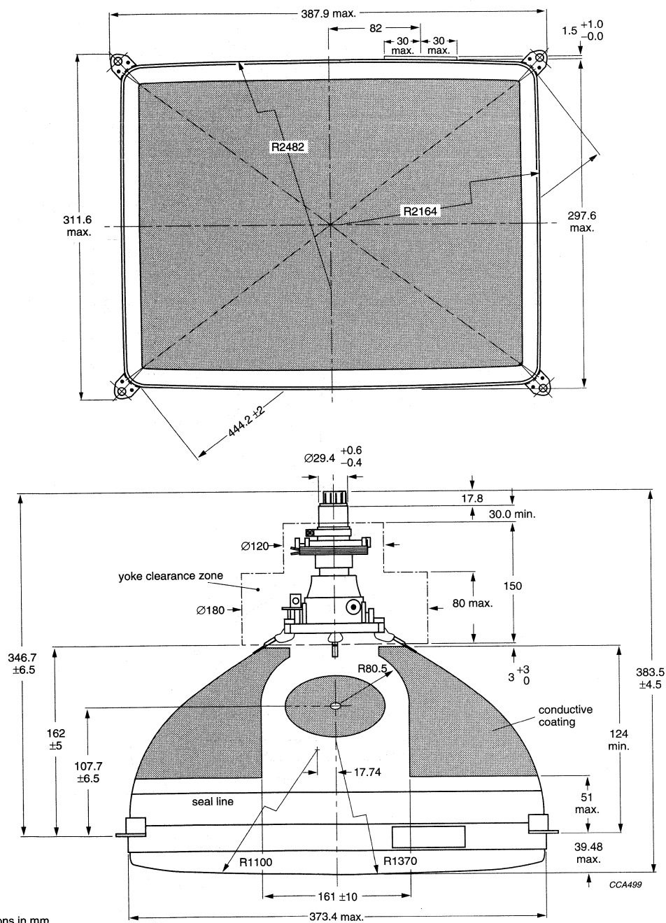
Fig.12 Top view.
