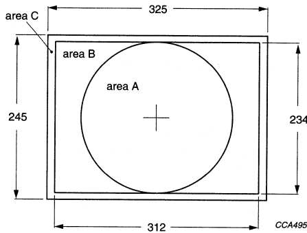
Fig.2 Maximum misconvergence.
