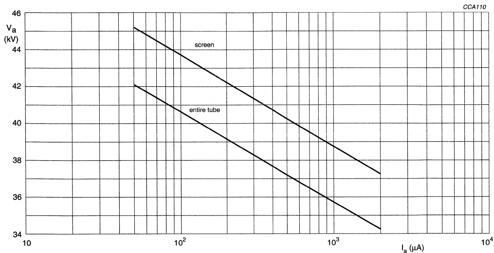
Fig.15 1 \mu\text{Sv/h} iso-exposure-rate limit curve.
