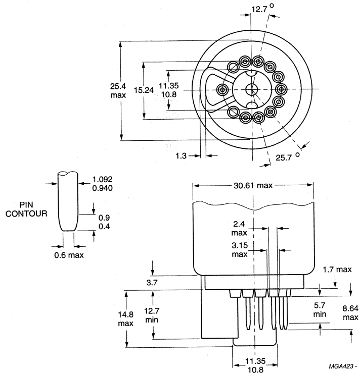
Fig.9 JEDEC B10-277 configuration.
