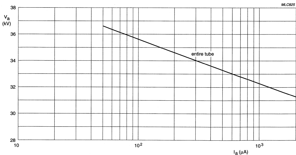
Fig.22 0.5 mR/h iso-exposure-rate limit curve.
