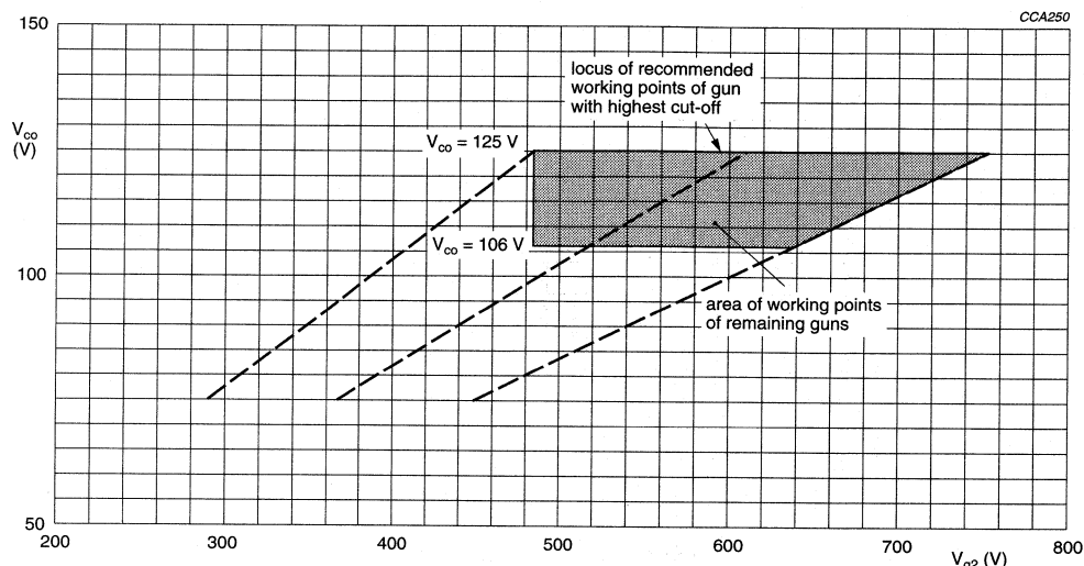
Fig.18 Raster cut-off design chart.
