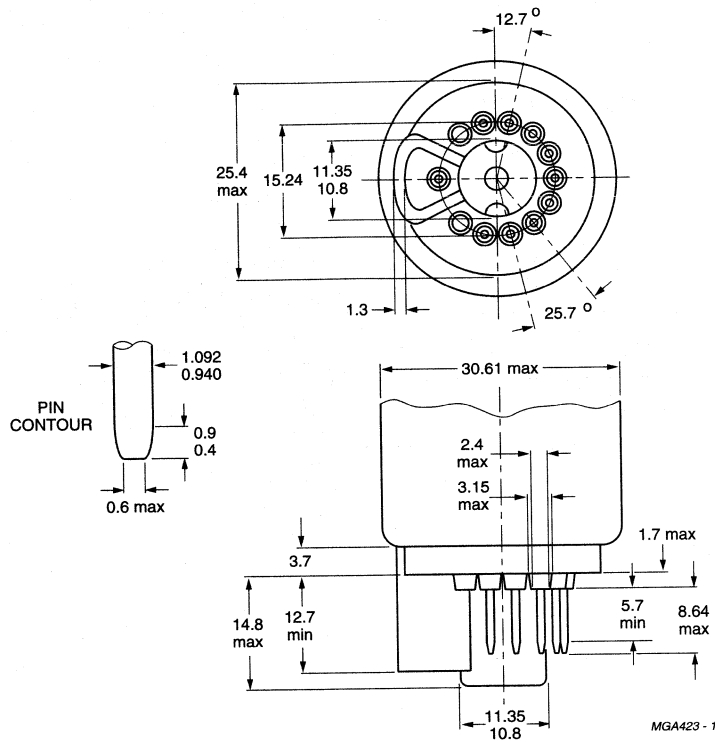
Fig.12 JEDEC B10-277 configuration.
