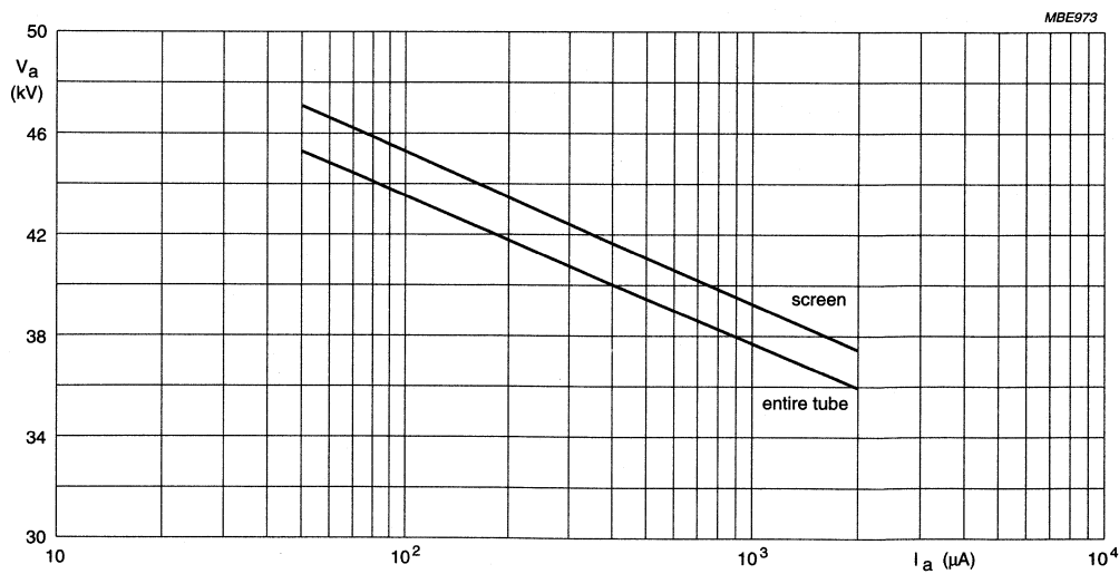
Fig.14 Iso-exposure-rate limit curves at 0.5 mR/h.
