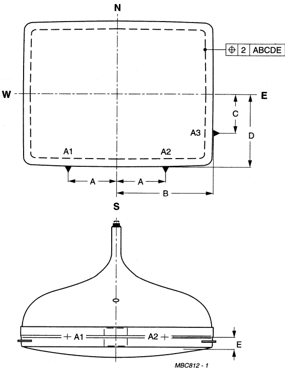
Fig.1 Phosphor alignment.
