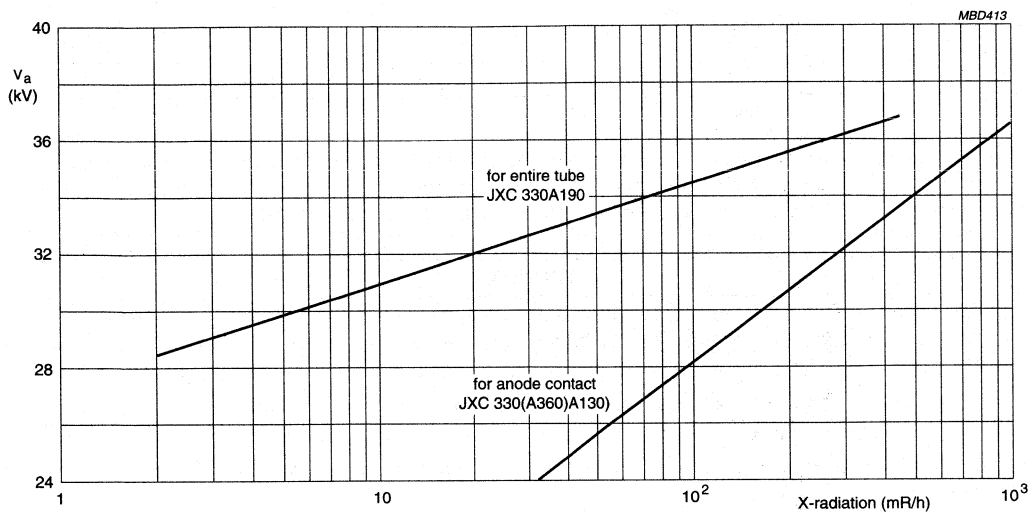
Fig.27 X-radiation limit curve at a constant anode current of 300 \mu\text{A} .
