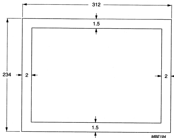
Fig.5 General distortion.
