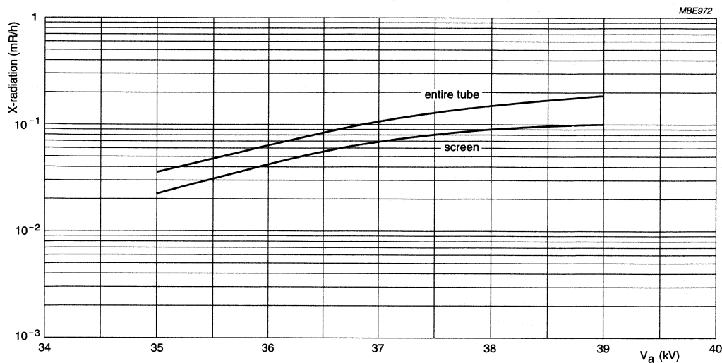
Fig.13 X-radiation limit curves at a constant anode current of 300 \mu A.
