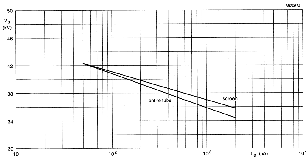
Fig. 15 Iso-exposure-rate limit curves at 0.5 mR/h.
