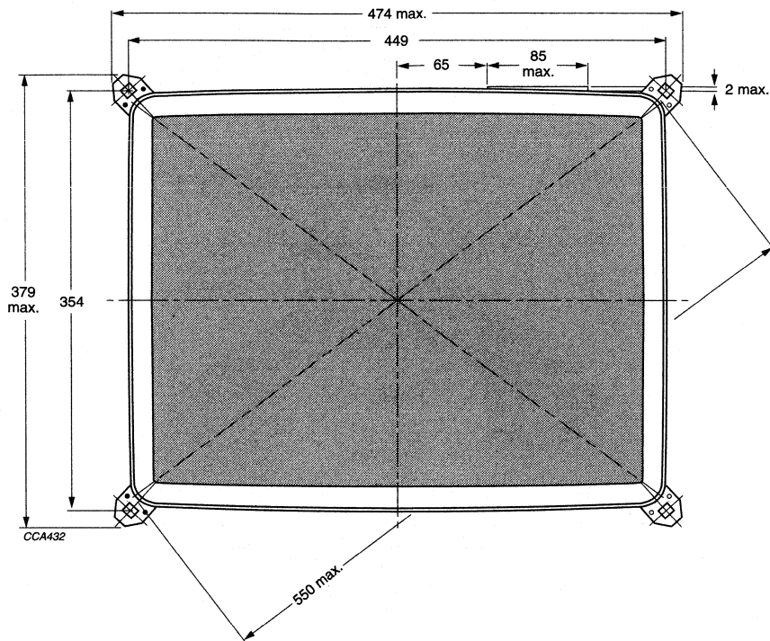
Fig.15 Tube dimensions; front view.
