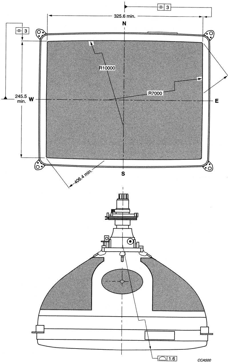
Fig.13 Dimensions of phosphor area on screen.
