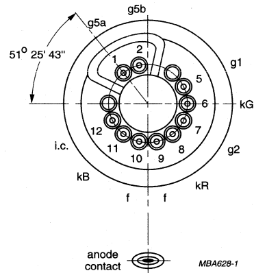
Fig.7 Pin arrangement.
