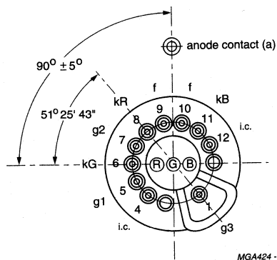
Fig.13 Pin configuration.
