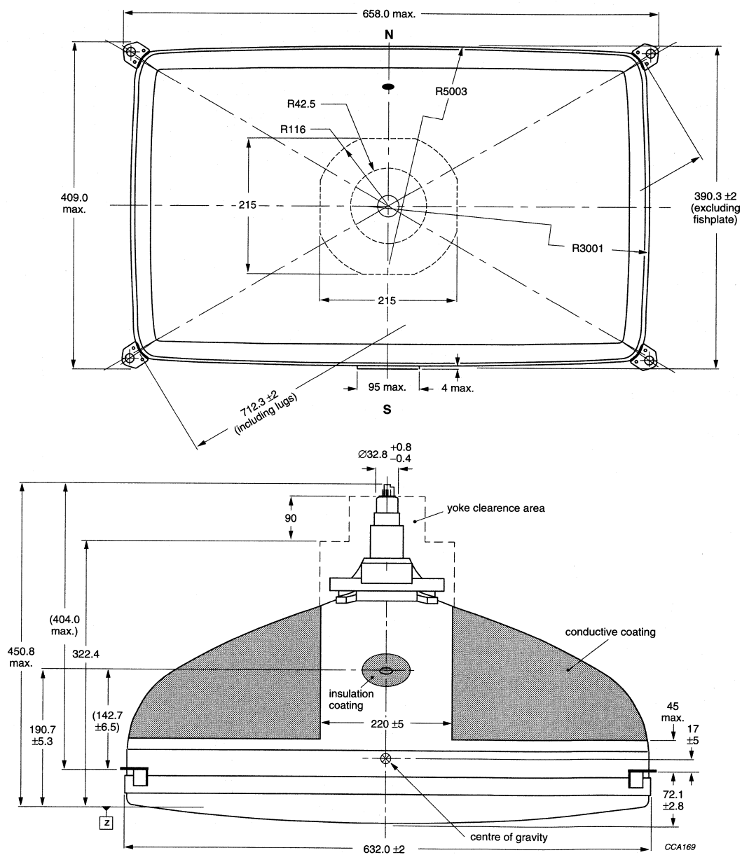
Fig.1 Assembly dimensions.
