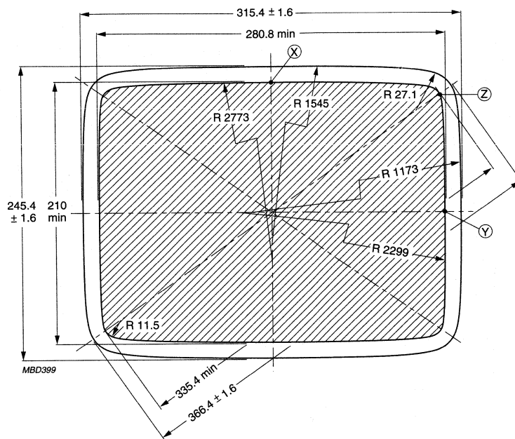
Fig.17 Screen dimensions.
