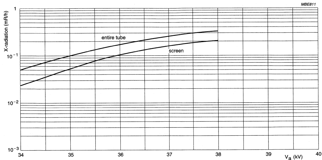
Fig. 14 X-radiation limit curves at a constant anode current of 300 \mu A.
