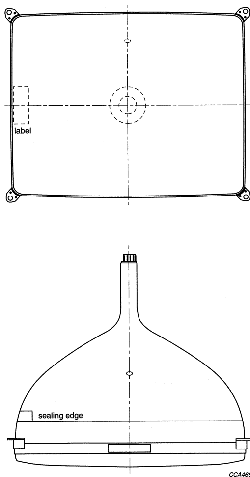
Fig.27 Label positioning.
