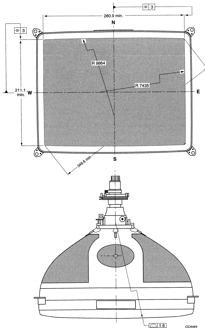
Fig.14 Screen dimensions.
