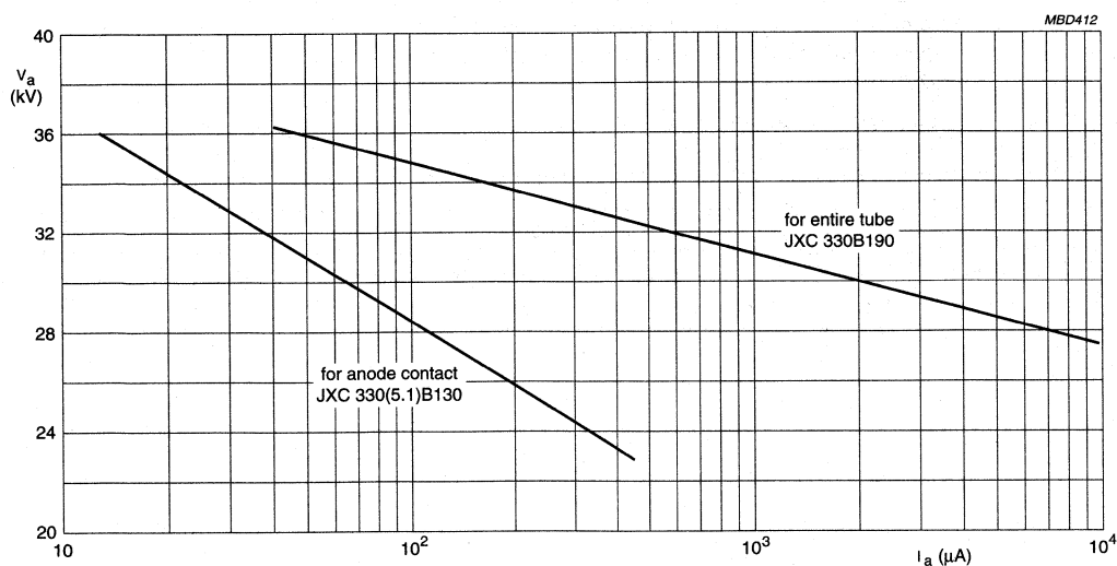
Fig.28 0.5 mR/h iso-exposure-rate limit curve.
