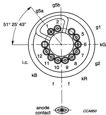
Fig.10 Pin arrangement.
