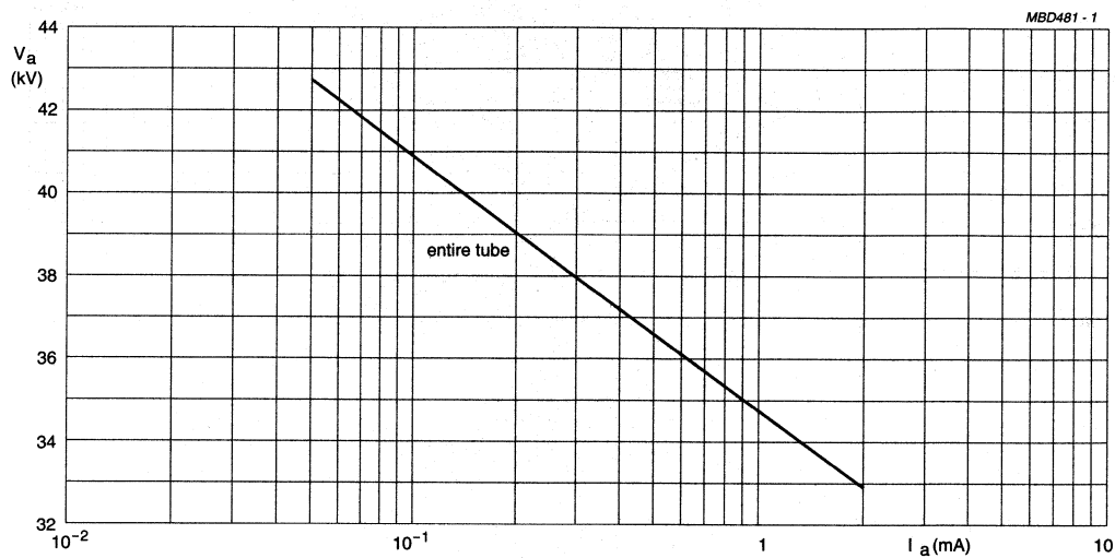
Fig.16 0.5 mR/h iso-exposure-rate limit curve.
