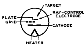
ELECTRON-RAY TUBE
