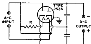
R = HEATERS OF OTHER TUBES IN SERIES WITH VOLTAGE-DROPPING RESISTOR
