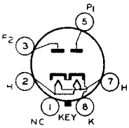
G-6S
