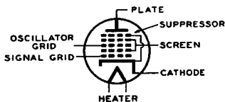
PENTAGRID MIXER
