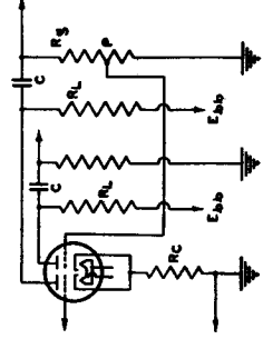
TWIN-TRIODE DIAGRAM WITH LEGEND
