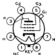
G-7R (6K7-G)
