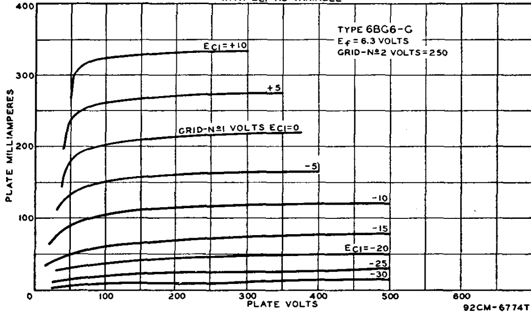
AVERAGE PLATE CHARACTERISTICS WITH E_{C1} AS VARIABLE
