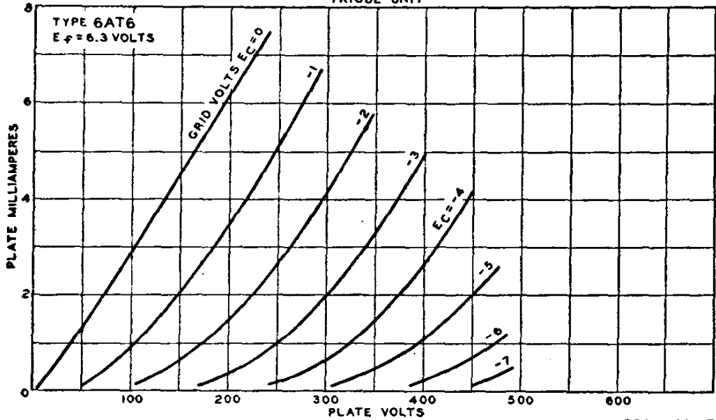
AVERAGE PLATE CHARACTERISTICS TRIODE UNIT
