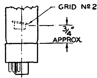
Location of Grid No.2 in Tube Neck.
