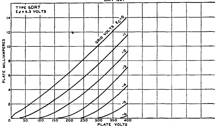
AVERAGE PLATE CHARACTERISTICS UNIT N°1
