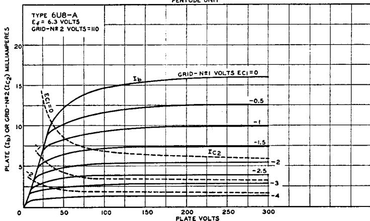
AVERAGE CHARACTERISTICS PENTODE UNIT
