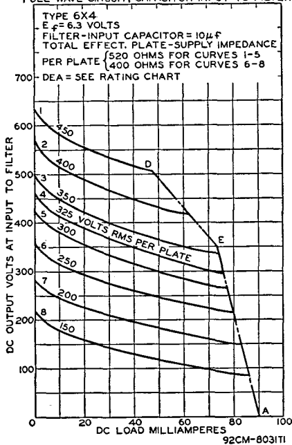
OPERATION CHARACTERISTICS FULL-WAVE CIRCUIT, CAPACITOR INPUT TO FILTER
