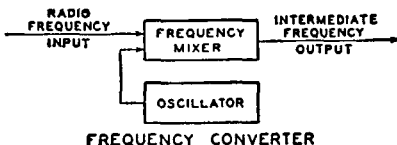
Fig. 77—Block diagram of simple frequency-converter circuit.
