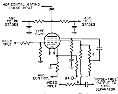
Fig. 43—Typical noise-cancellation circuit.
