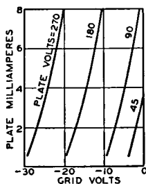
Fig. 12—Family of transfer-characteristic curves.
