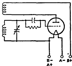
Fig. 67—Tuned-grid triode oscillator circuit using filament-type tube.
