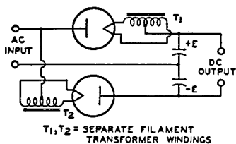
Fig. 46—Full-wave voltage-doubler circuit.
