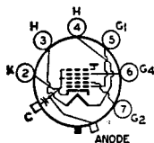
7FA ANODE = G 3 + G 5 + C1 FOCUSING ELECTRODE = G 4
