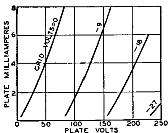
Fig. 11—Family of plate-characteristic curves.
