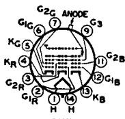
14AH ANODE = G_4 + G_5 + CL + R FOCUSING ELECTRODE = G_3
