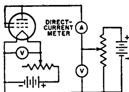
Fig. 100—Fundamental circuit of an emission tester.
