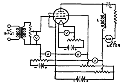
Fig. 103—Fundamental circuit of a power-output tester for class A operation of tubes.
